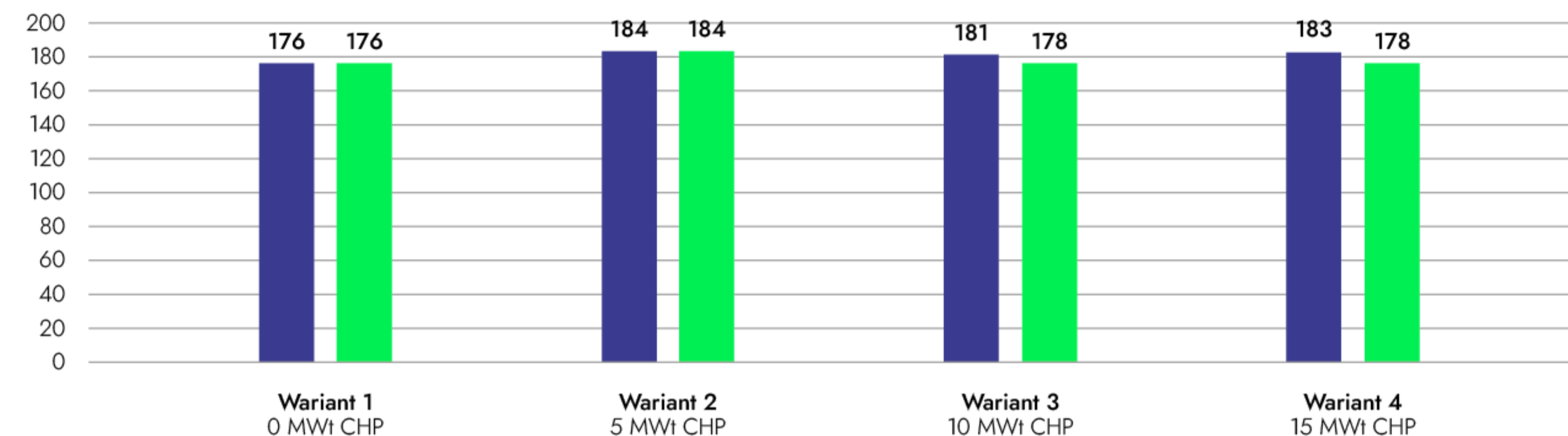
LCOH [PLN'25/GJ] Rynek 35 MW
